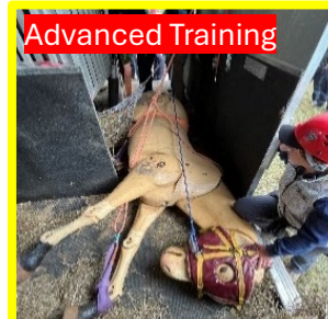
Horse Down in Trailer
